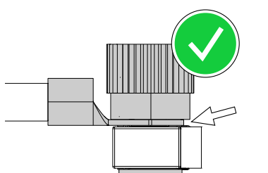
Illustration 79. Montage correct
